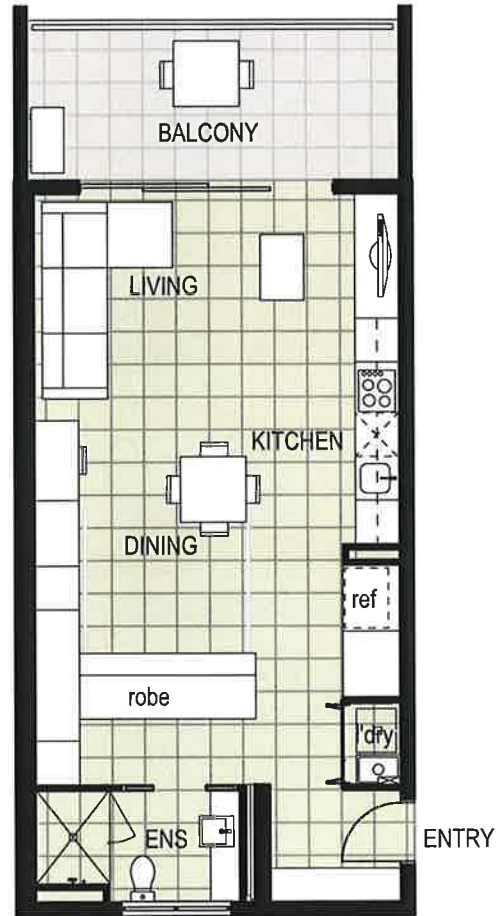
ALTERNATIVE LAYOUT FLOOR PLAN
